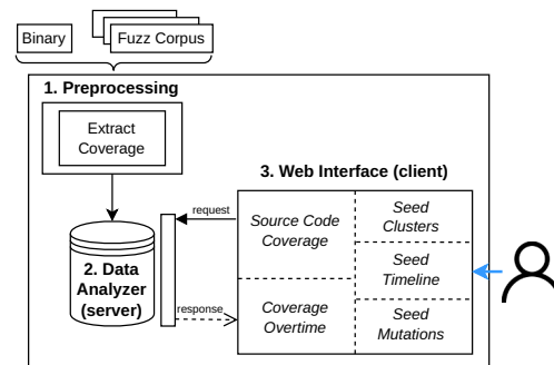
Fig. 1: High-level architecture and workflow of SEEDUI.
